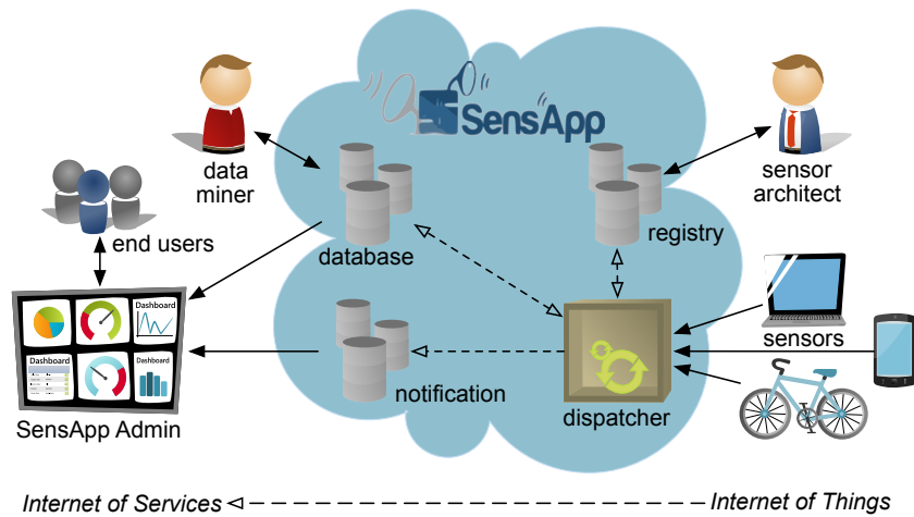
Figure 3: The SENSAPP architecture [22]
